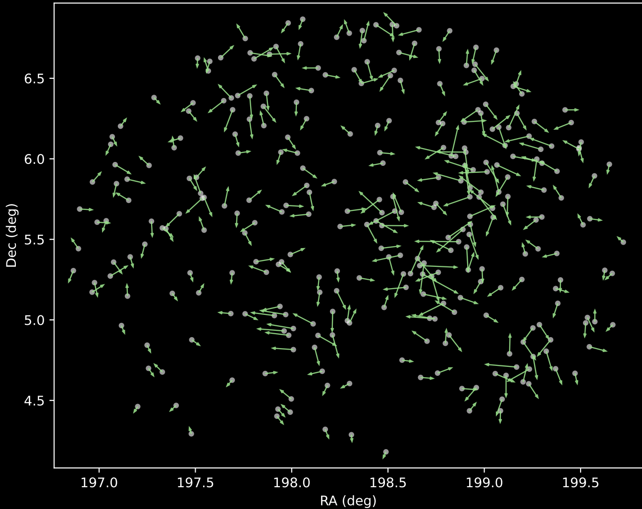
APOGEE DR17 Cluster 5 Proper Motion Vectors (n=303)
