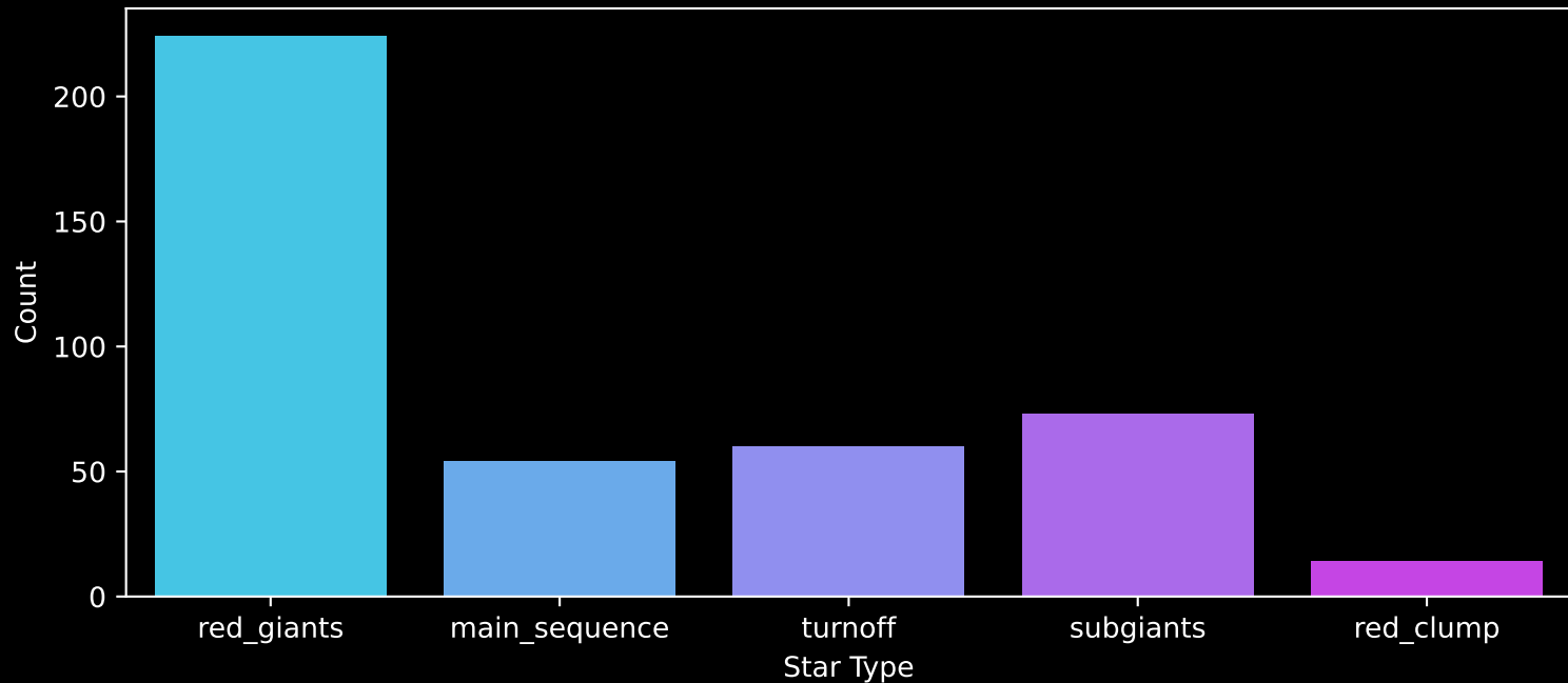
APOGEE DR17 Field: [HD46375] Count plot of Star Type
