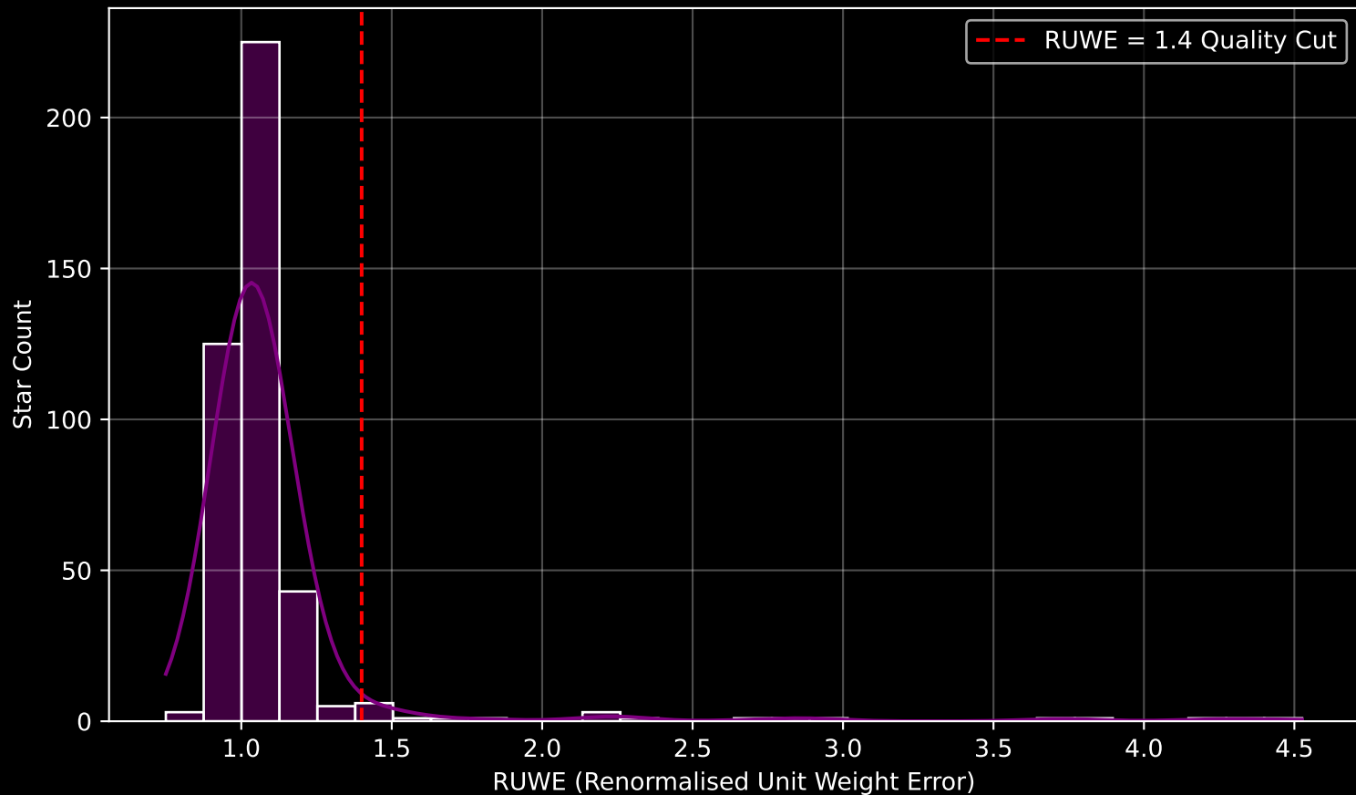
GAPOGEE DR17 Field [HD46375] RUWE Distribution (n= 422)
