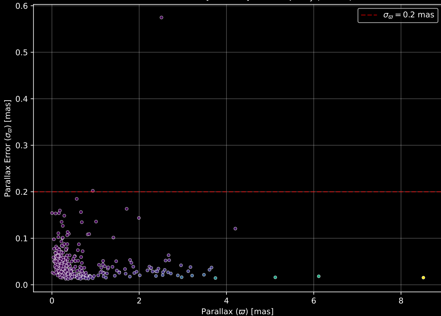
APOGEE DR17 Field: [HD46375] Parallax Quality (n= 425)
