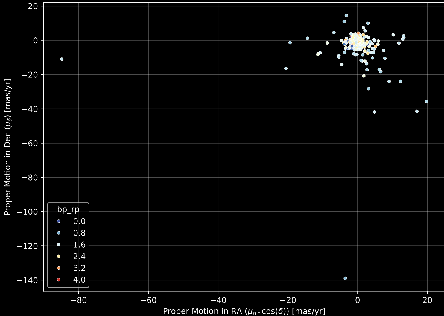
APOGEE DR17 Field: [HD46375] Proper Motion Diagram (n= 425)
